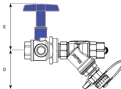
Maple Connect FCU ML-CFCUT - side view
