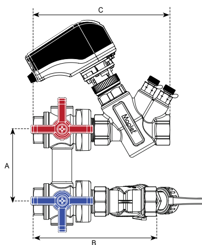
Maple Connect FCU ML-CFCUT - top view
